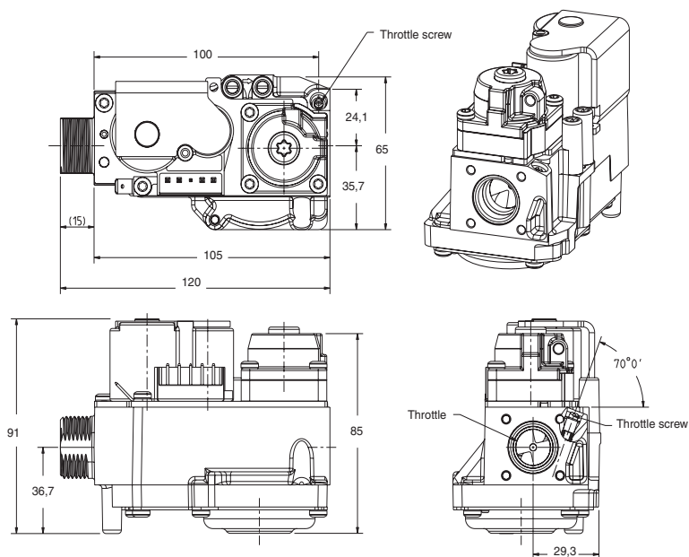
Dimensional drawing VK41.5VE/VK81.5VE (Throttle)
